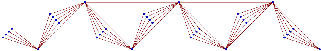
FIGURE 1. The graph P(3, 5, 4)
