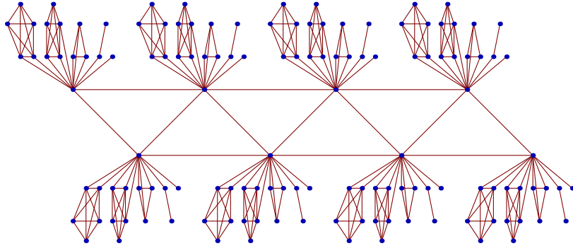
FIGURE 2. The case \vec{m} = (5, 5, 3, 2, 1) and \vec{u} = (2, 3, 3, 1, 1)
