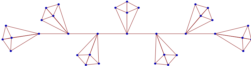
FIGURE 1. The graph P(2, 6) \nabla(K_4 - e, V(K_4 - e))
